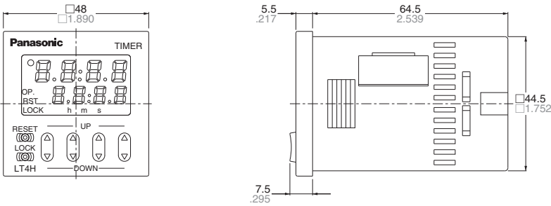
Screw terminal type (Flush mount)
