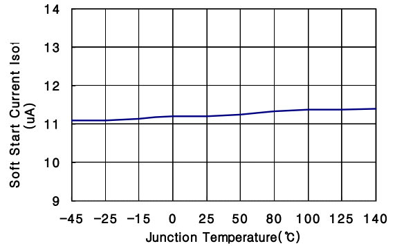
Figure 14. Soft-Start Current
