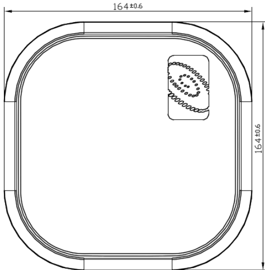
Wall Mount to Antenna - Front View
