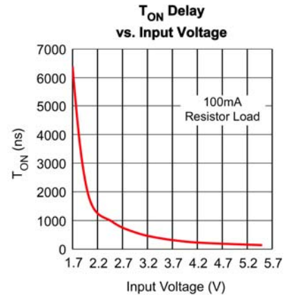
MIC94080/1
